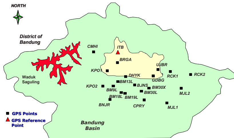
Figure 3. GPS subsidence monitoring network in Bandung basin.
