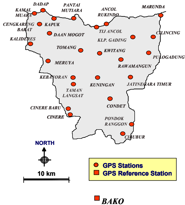
Figure 2. GPS subsidence monitoring network in Jakarta.
