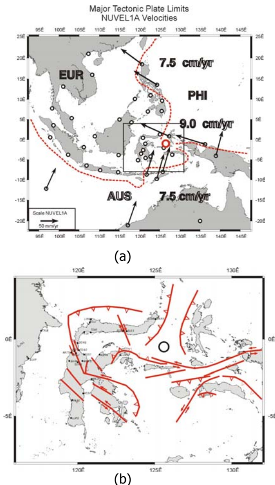
Figure 1: (a) Sulawesi in Major tectonic Plates; (b) Main tectonics in Sulawesi
