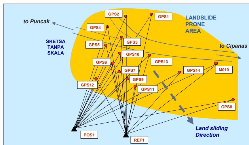
Figure 4. GPS landslide monitoring network in Megamendung area.
