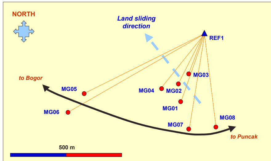
Figure 5. GPS landslide monitoring network in Megamendung area.
